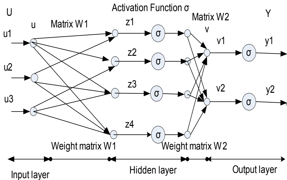
Figure 3: 3-4-2 neurons detailed multilayer perceptron architecture
