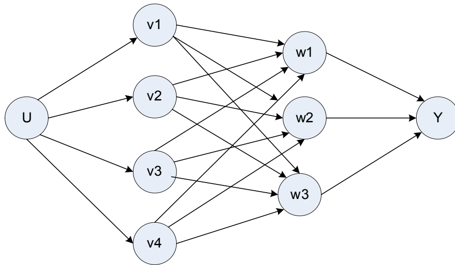
Figure 2: 1-4-3-1 neurons simplified multilayer perceptron architecture
